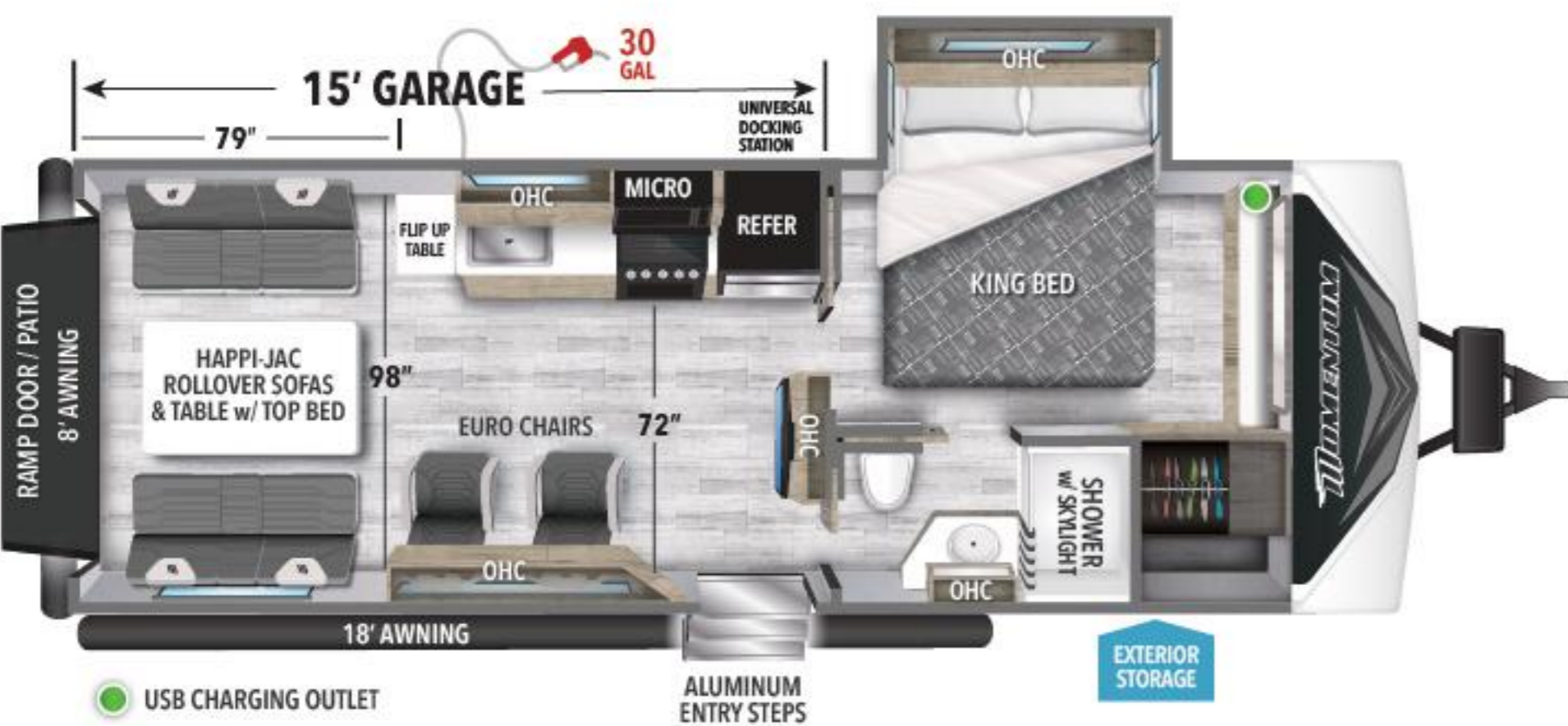
23G 15' GARAGE UVW' EMPTY HITCH' GVWR LENGTH' HEIGHT CAPACITY 6,897 1,266 13,000 28' 10" 12' 4" 96 74 39
