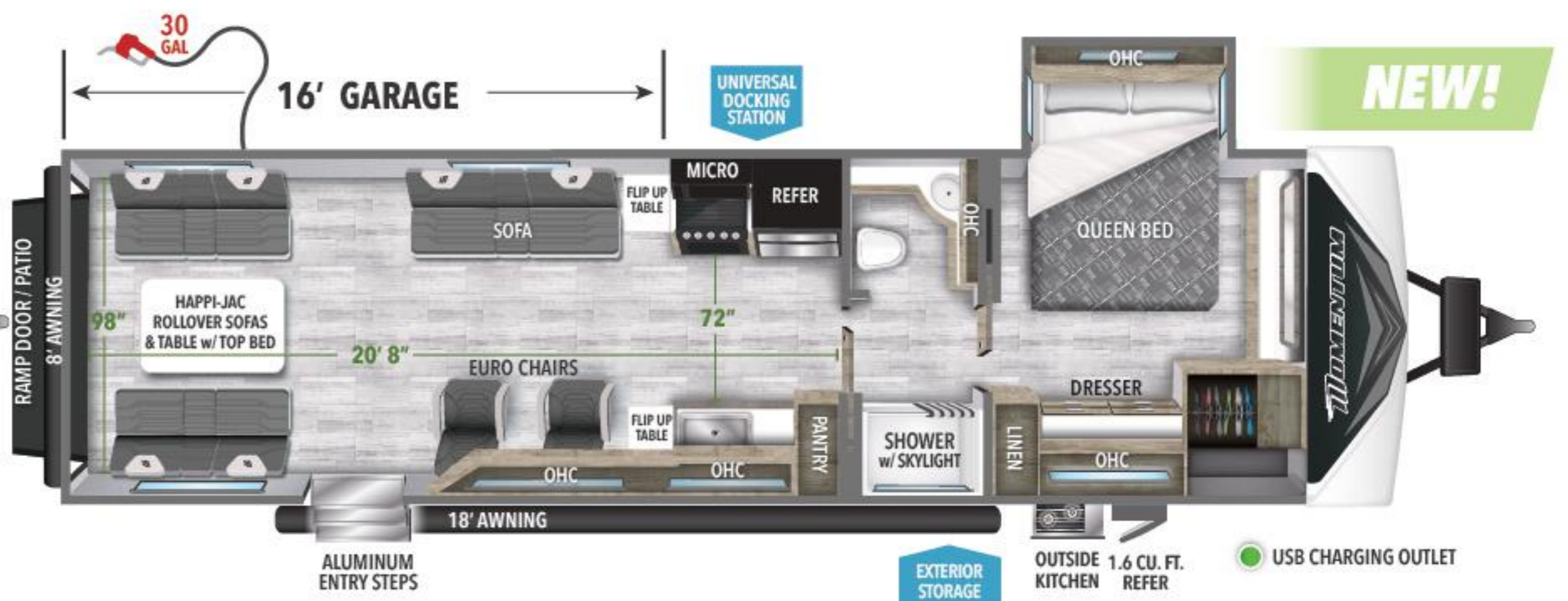
32G 16' GARAGE UVW' EMPTY HITCH' GVWR LENGTH' HEIGHT CAPACITY 9,374 1,320 13,000 36' 10" 12' 4" 100 78 39
