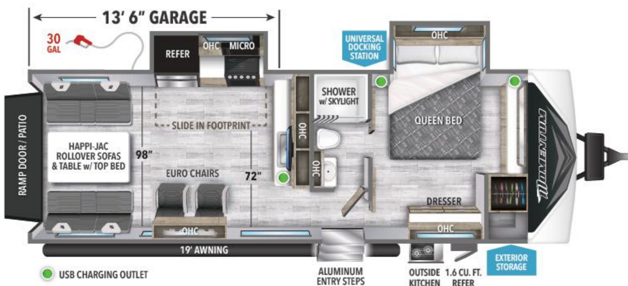
25G 13' 6" GARAGE UVW' EMPTY HITCH' GVWR LENGTH' HEIGHT CAPACITY 7,900 1,150 13,000 30' 11" 12' 4" 96 78 39
