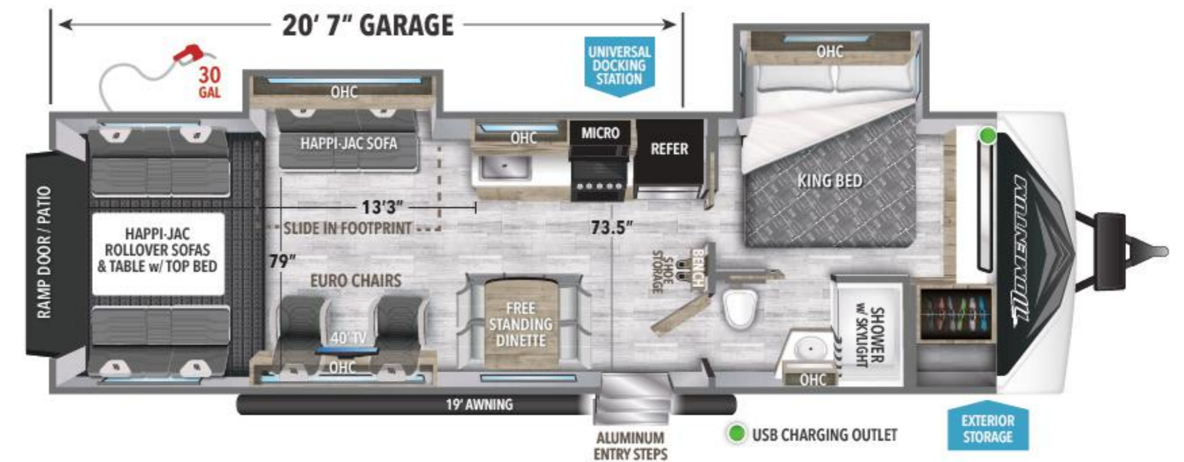
30G 20' 7" GARAGE UVW' EMPTY HITCH' GVWR LENGTH' HEIGHT CAPACITY 8,800 1,350 13,000 34' 11" 12' 4" 96 76 37
